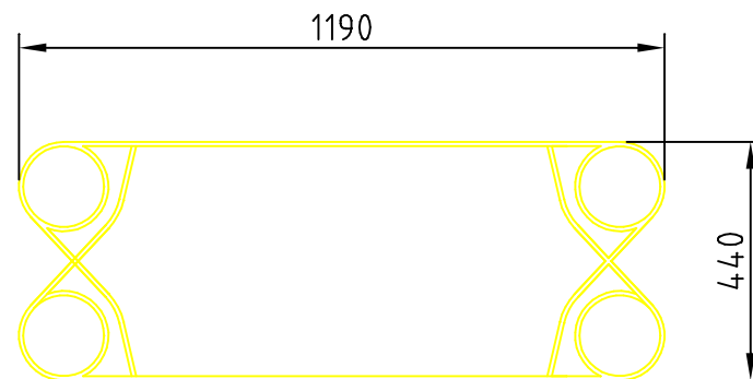
G-125, GASKET
