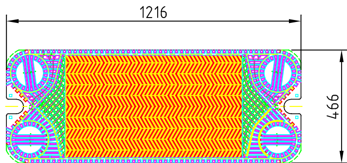
SHE-125, PLATE
